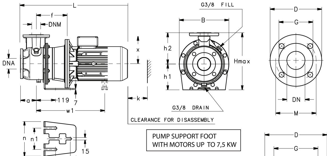
PUMP FLANGES
