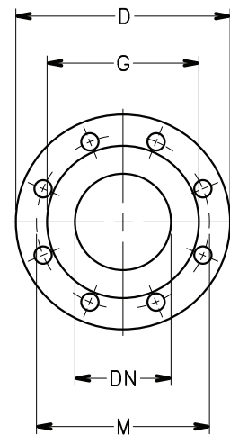
PUMP FLANGES
