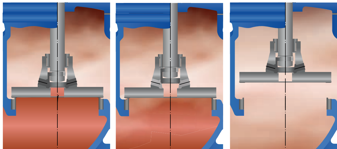
Phase 1: The valve is completely closed
