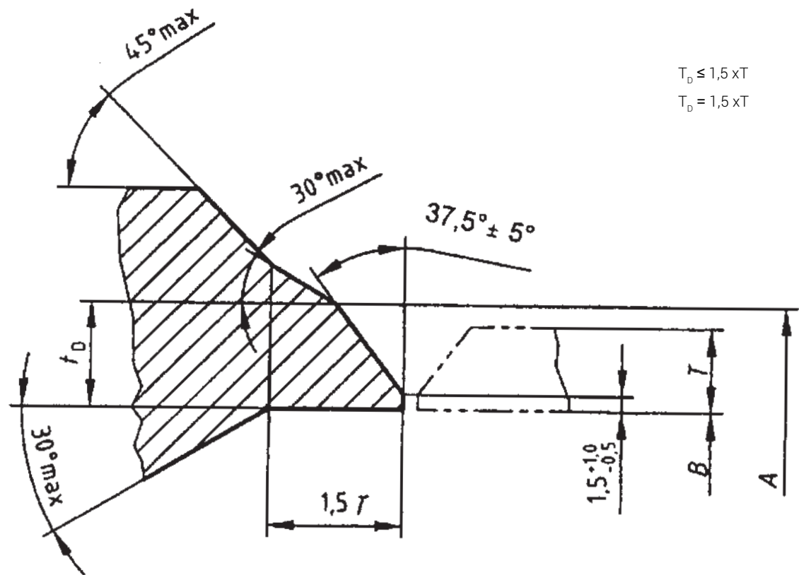
Single-V butt weld end connection to pipe of wall thickness 4 mm ≤ 22 mm
