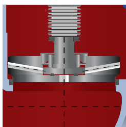
Balanced plug
