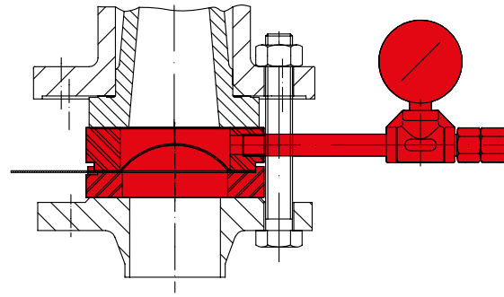
Rupture disc
