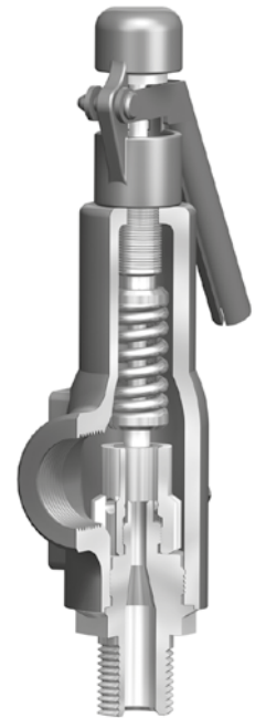
Fig. 969 open lifting device
