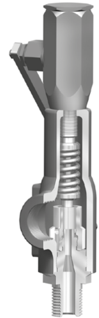
Fig. 966 closed lifting device
