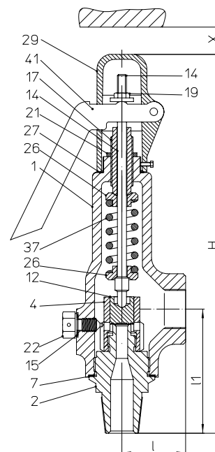
Fig. ... 969 open lifting device
