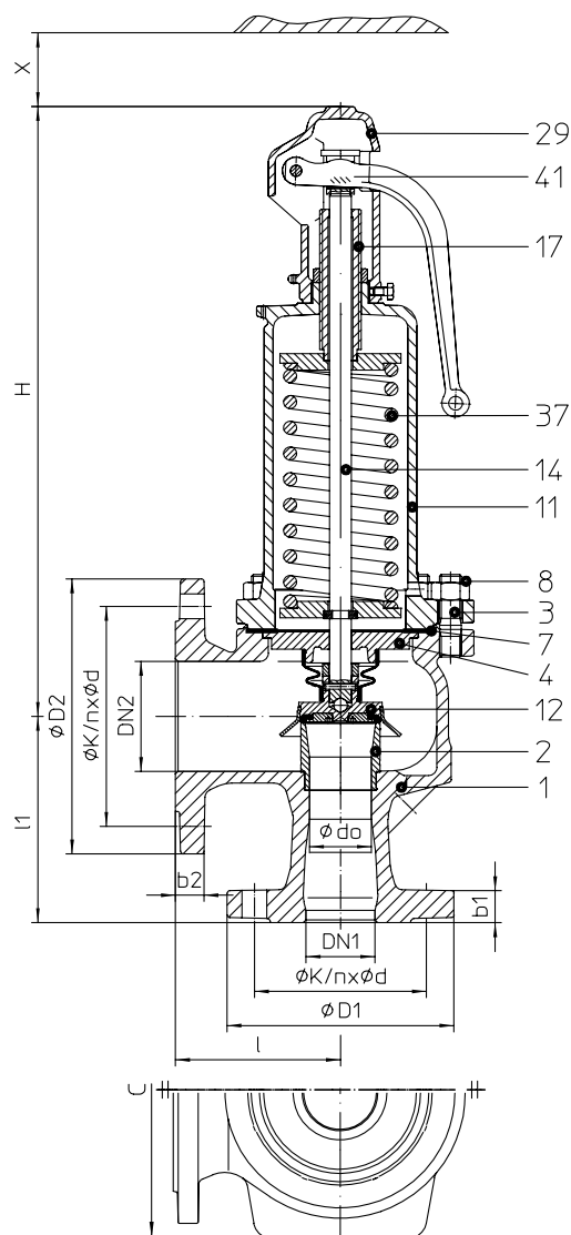
Fig. ... 903 open lifting device, closed bonnet
