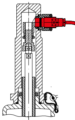
Proximity switch
