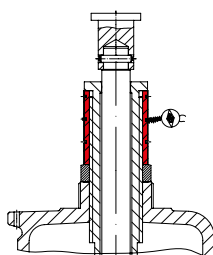
Lock bush
