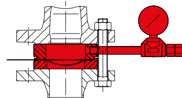
Rupture disc
