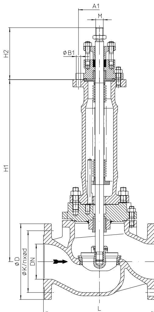
Fig. 471 DN125-150 (e.g.: DP34T-35; AUMA 14.2)
