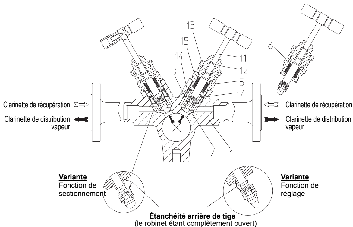
Fig. 2: CODI®S - BR671/672 PN40-63 / Class 150 / Class 300 raccordement principal DN25-50 / raccords secondaires DN15-25
