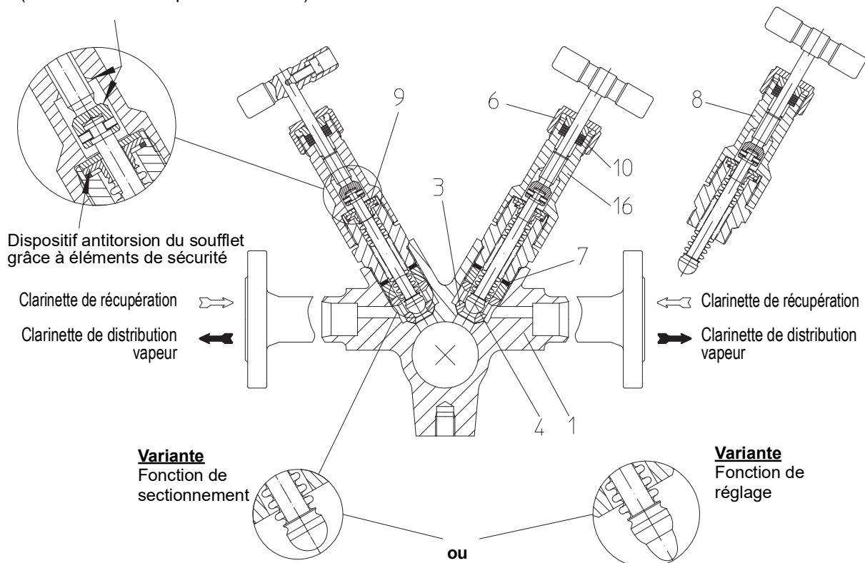
Fig. 3: CODI®B - BR675/676 PN40-63 / Class 150 / Class 300 raccordement principal DN25-50 / raccords secondaires DN15-25
