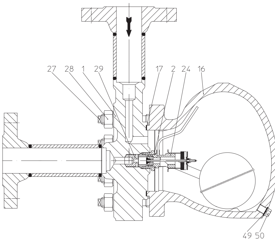
obr. 4: CONA ® S - BR632 PN160 DN15-50 Class 900 NPS 1/2"-2"
