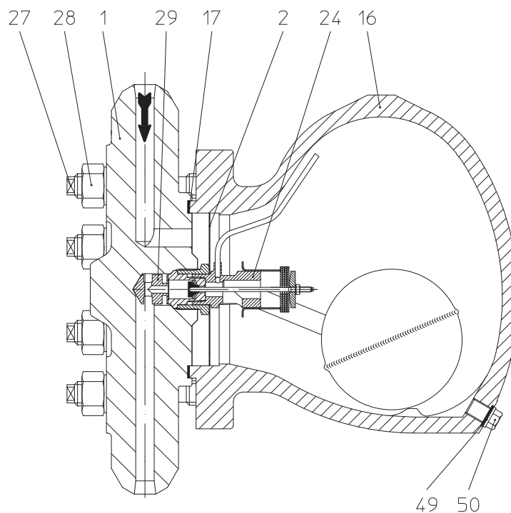
obr. 3: CONA ® S - BR631 PN160 DN15-50 Class 900 NPS 1/2"-2"
