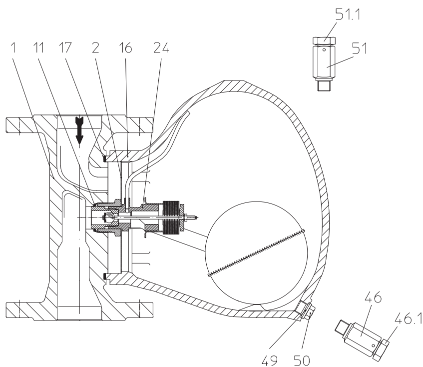
obr. 1: CONA ® S - BR631 PN16-40 DN15-50 Class 125 / Class 150 / Class 300 NPS 1/2"-2"
