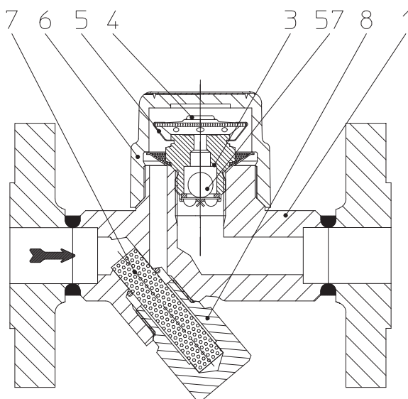
obr. 5: CONA ® M - BR613 PN40 / Class 150/300
