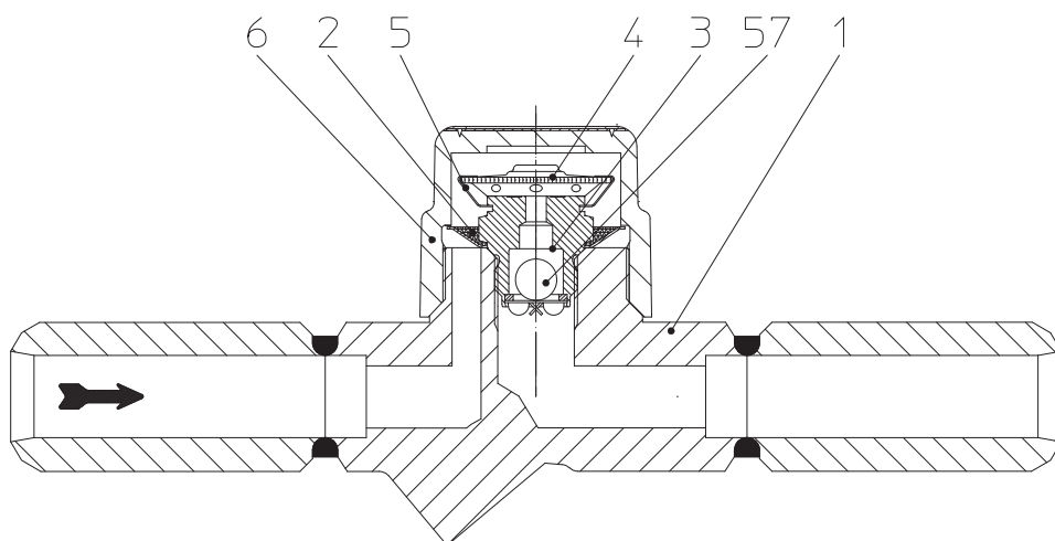
obr. 4: CONA ® M - BR611 PN40 / Class 150/300
