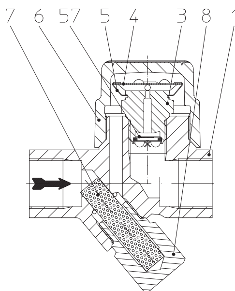
obr. 3: CONA ® M - BR612 PN40 / Class 150/300
