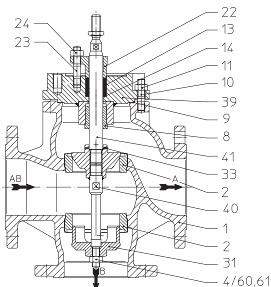
Рис. 7: BR 450 DN125v-150v
