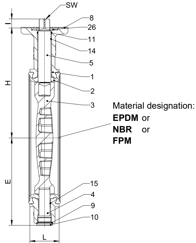
Fig. 1: Butterfly valve
