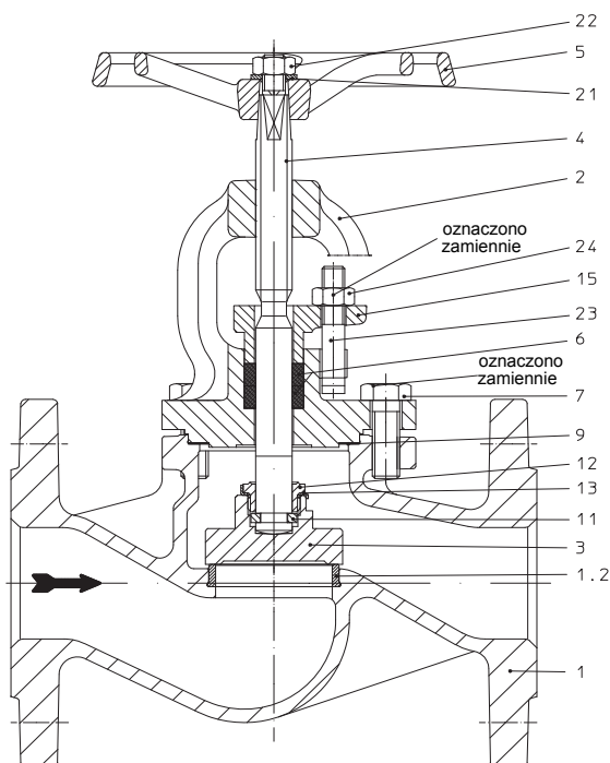
Rys. 3: STOBU-DG EN-JL1040/JS1049
