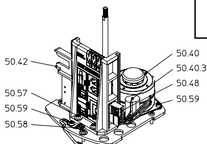
Synchronous motor 230 V AC
