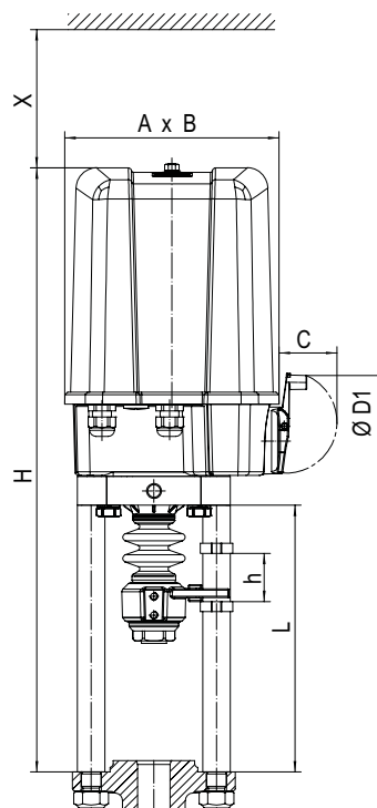
2,2 - 5 kN (495 - 1124 lbf) Nominal travel > 1.18 in - 1.97 in
