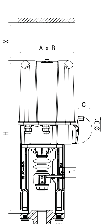
2,2 - 5 kN (495 - 1124 lbf) Nominal travel max. 1.18 in
