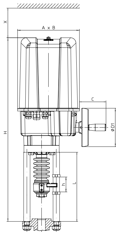
12 - 25 kN (2698 - 5620 lbf) Nominal travel max. 3.15 in
